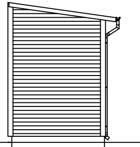
GAVELFASAD
